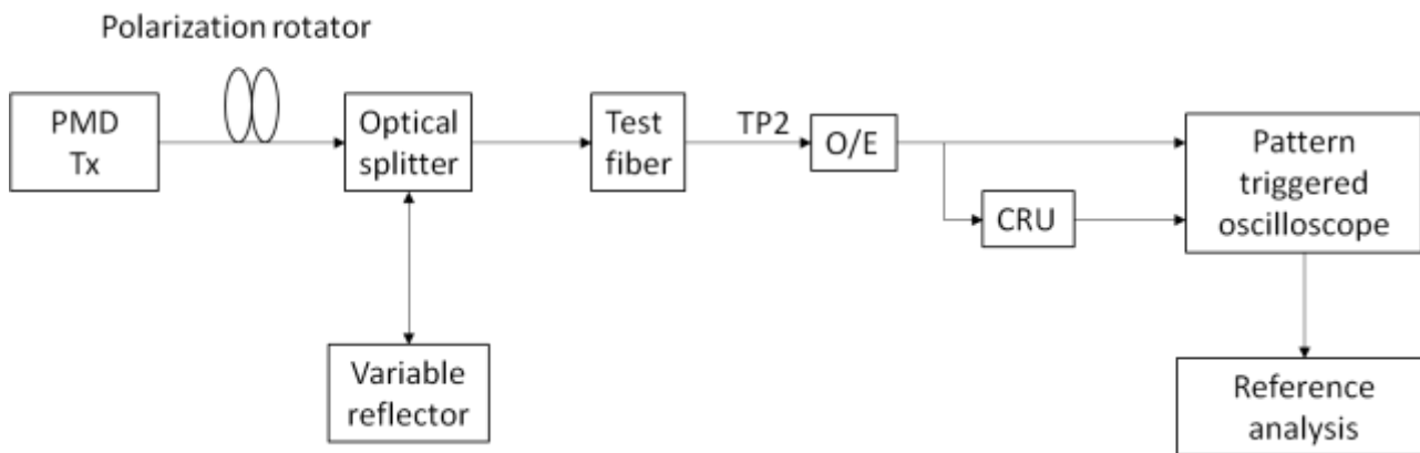
Figure 5-3: Test set up for 200G-LR4-Open Eye transmitter output
