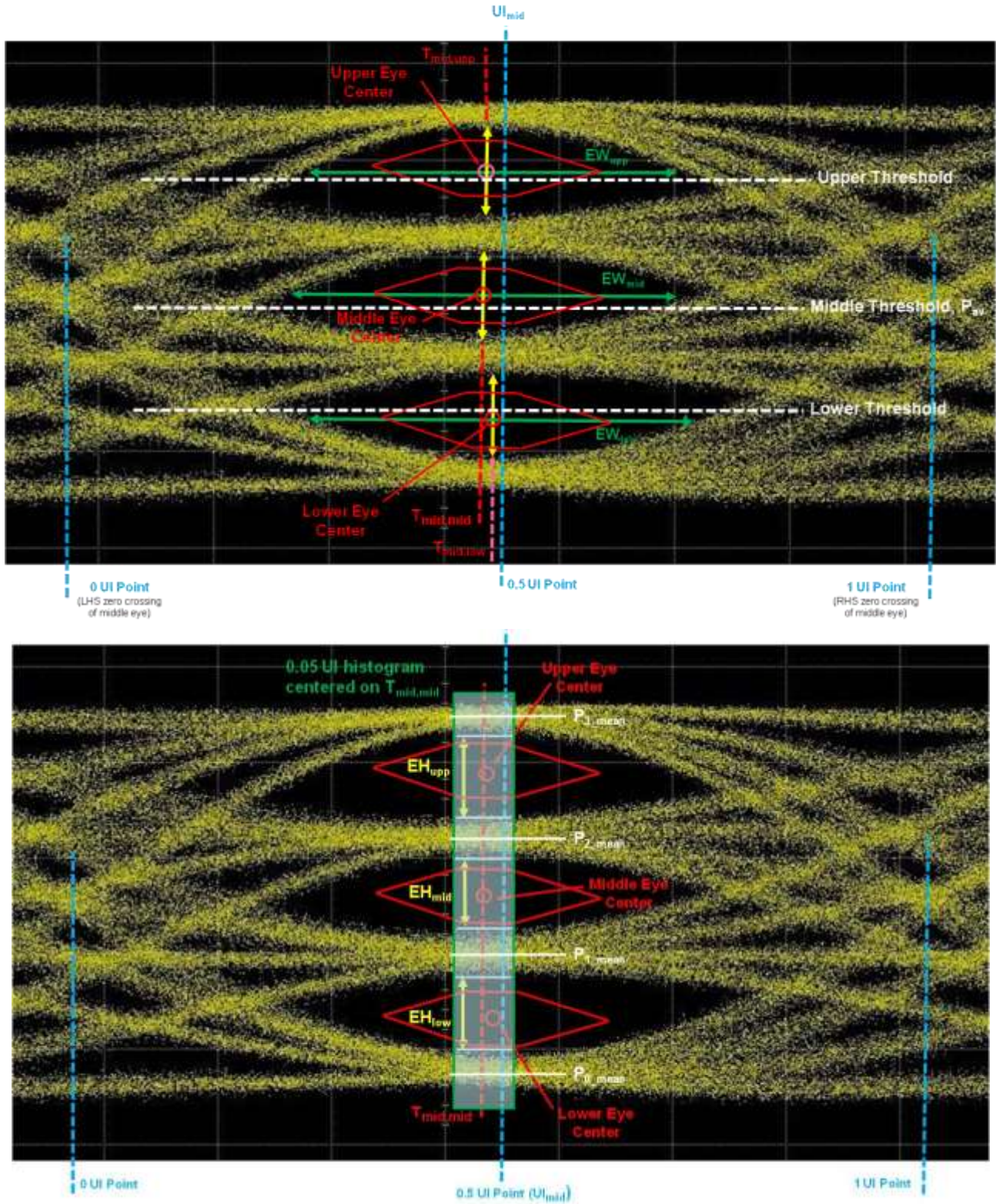
Figure 5-4: TP2 PAM4 Eye Parameters for 200G-LR4-Open Eye
