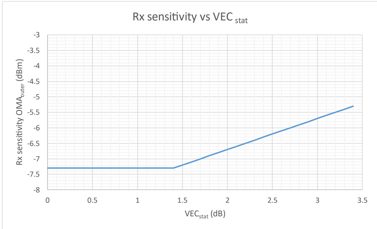
Figure 5-6: Receiver sensitivity as a function of VEC stat
