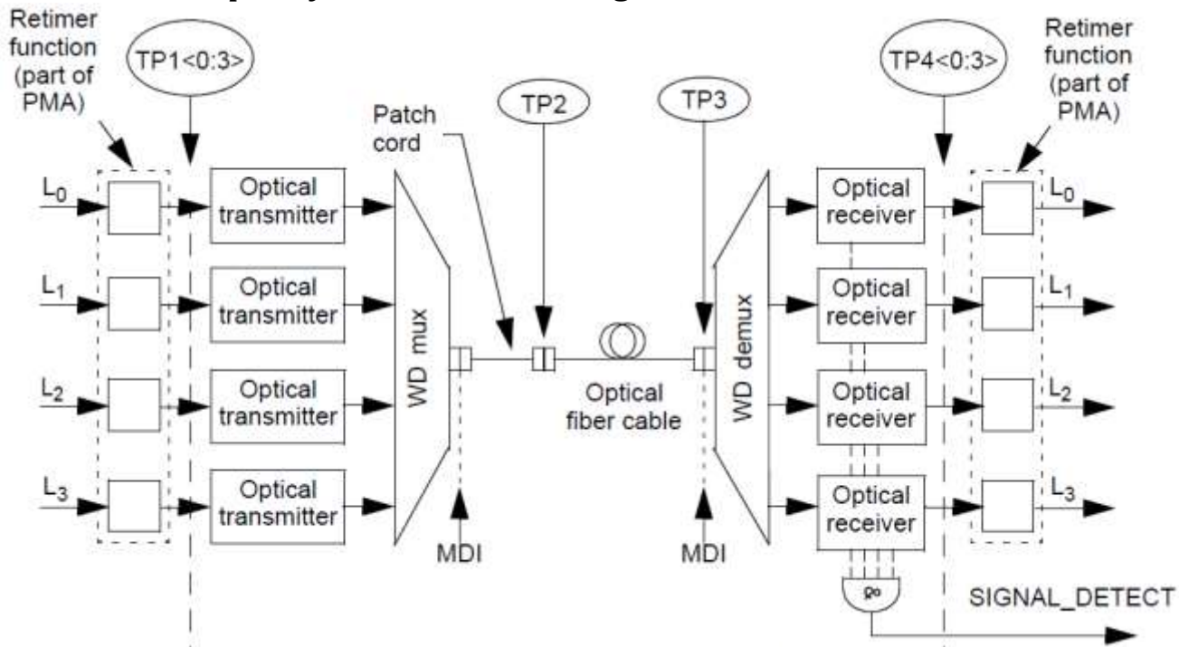
Figure 3-1: Block diagram for 200G-LR4-Open Eye transmit/receive paths
